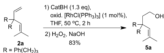
Scheme 3. Hydroboration of 2a with CatBH in a reaction catalyzed by partially oxidized [\text{RhCl}(\text{PPh}_3)_3] .
